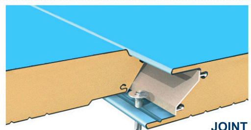
JOINT
