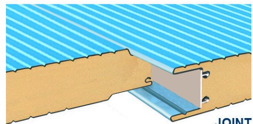
JOINT
