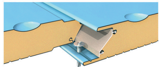
JOINT
